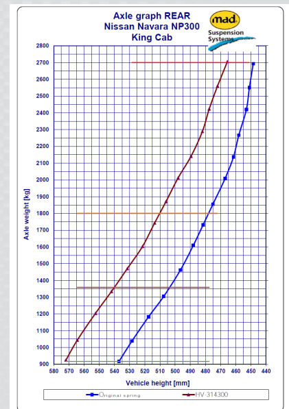
Power Spring Characteristic HV-314300
